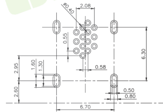
PCB LAYOUT (RECOMMENDED) (Tol: ±0.05)
