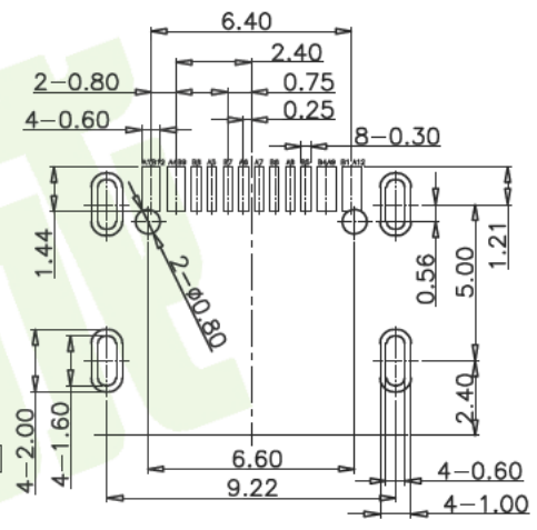
RECOMMENDED P.C.B. LAYOUT TOLERANCE UNSPECIFIED ±0.05mm
