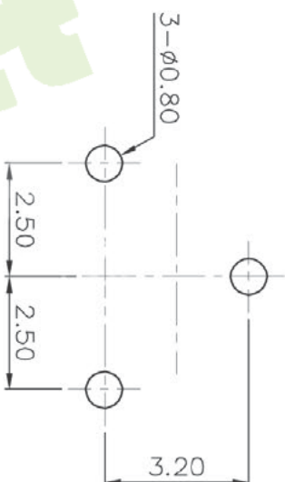
HOLE LAYOUT
