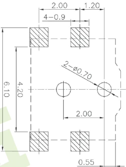
Recommended PWB piercing plan (Pitch tolerance \pm 0.05 )
