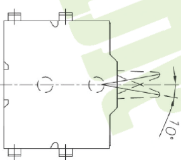
Recommended PWB piercing plan (Pitch tolerance \pm 0.05 )
