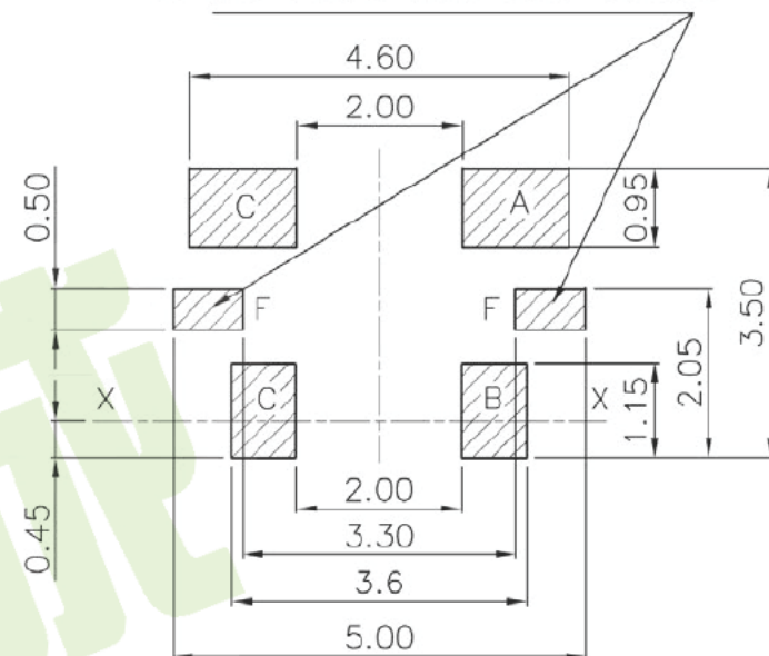
PCB Layout(Pattern Side)/A direction
