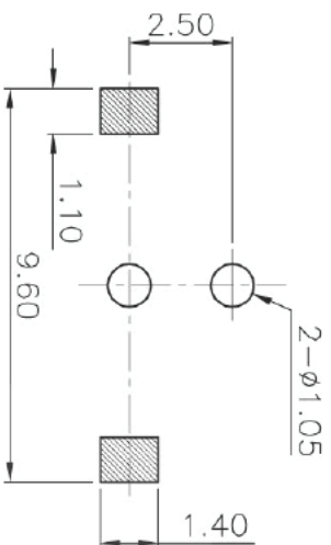
HOLE LAYOUT
