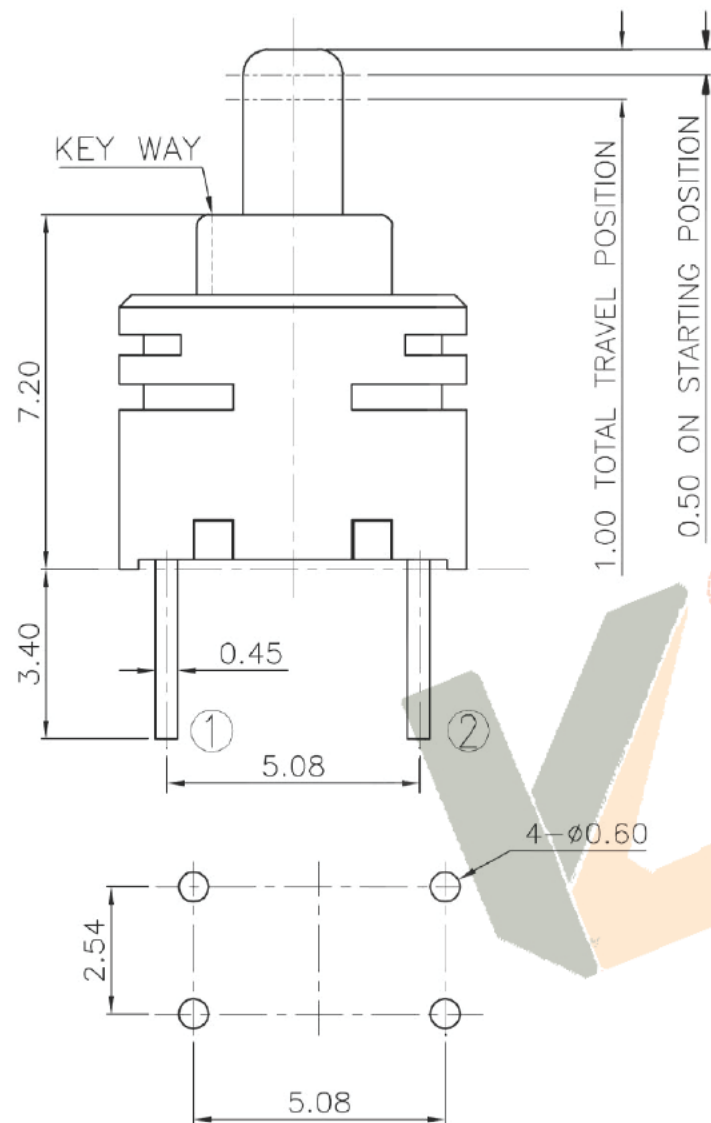
P.C. BOARD MOUNTING HOLE DIMENSIONS
