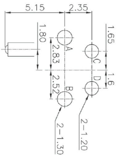
HOLE LAYOUT (TOP VIEW)
